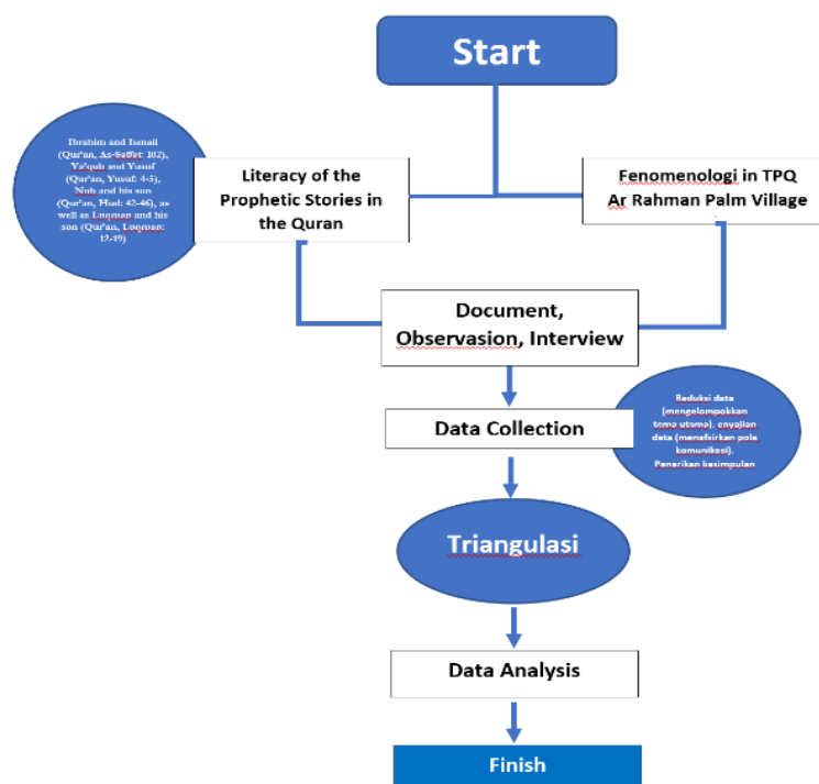
Gambar 1. Fowchart Penelitian
